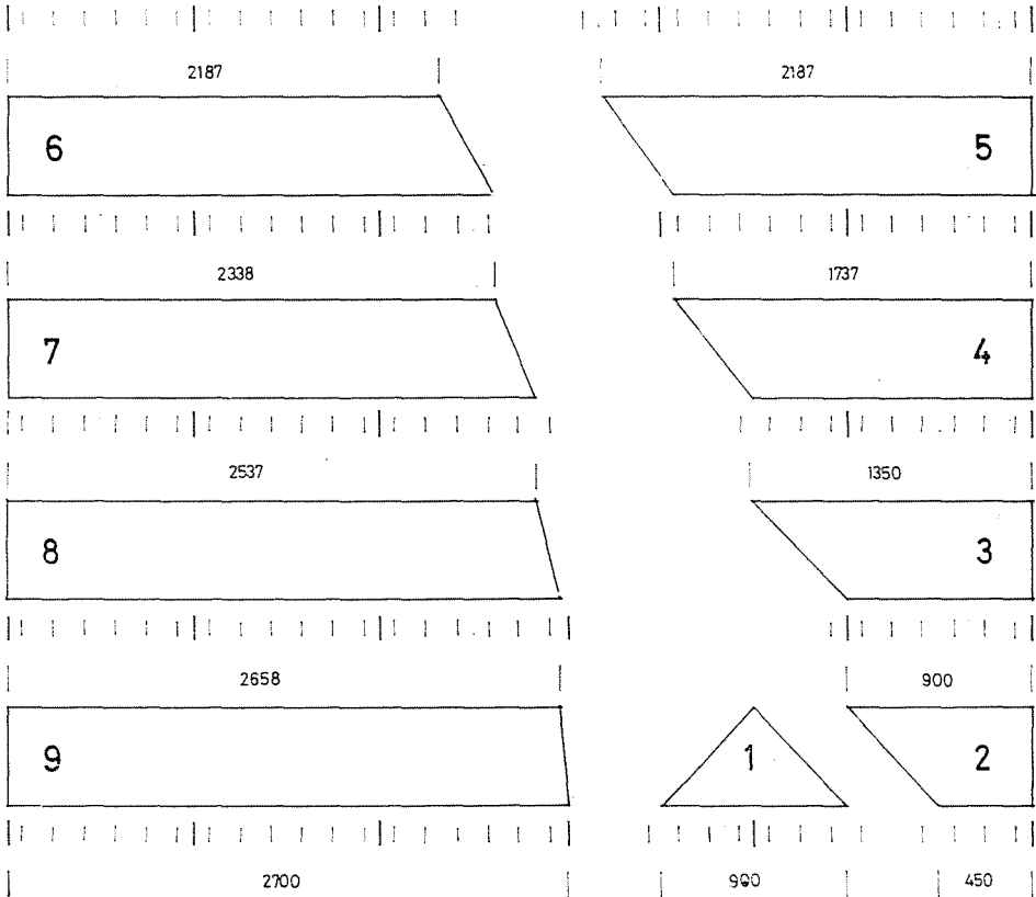
Fig. 16. Structural variation V. 2.: Basic tectonic elements (ribbed r.c. shell plane structural elements). Dimensions of the non-tectonic periodic gypsum surface elements with plane surface on both sides are identical with those of structural variation V. 1. (see: Fig. 12.)
