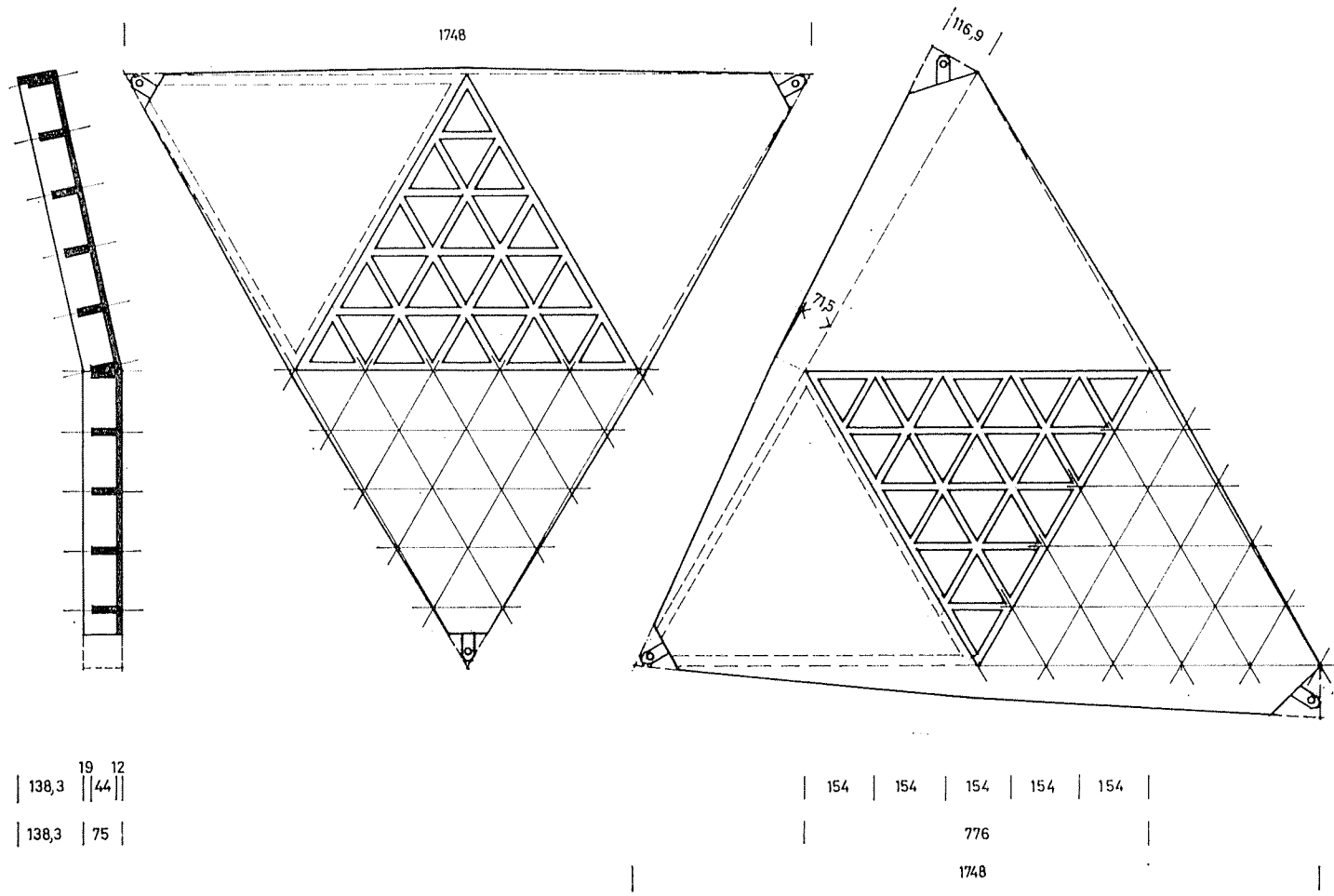
Fig. 34. Structural variation D. 2.: Basic non-tectonic and tectonic elements: The non-tectonic periodic triangular gypsum surface element (with plane surface on both sides) and the ribbed and folded r.c. shell structural small space-unit based on the "in-space" additivity of the non-tectonic periodic plane surface elements
