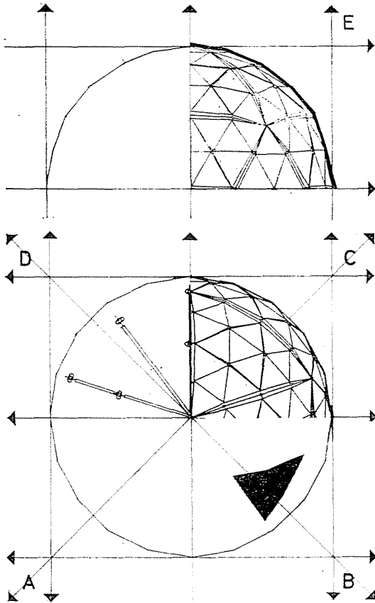
Fig. 33. The system of grids of variation D. 2. on plan and in section. Decomposition of the structure
