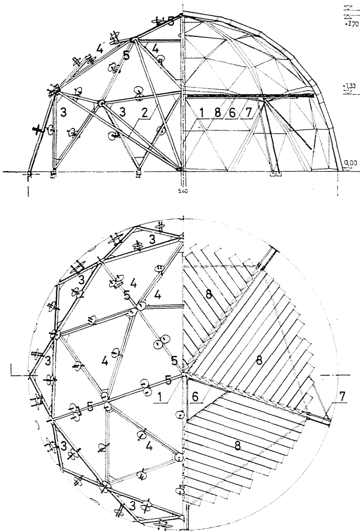
Fig. 32. Auxiliary structure and scaffolding for the assembly of the non-tectonic surface elements of variation D. 1. and for erection of the dome. Index: 1. Leading post started from the zero-level of co-ordination; 2. Stiffening radial etalon rods jointed to "collar" welded to leading post; 3, 4. Triangular elements of the auxiliary structure of different dimensions to point out location of the surface element and for supporting; 5. Linear elements of the auxiliary structure for the same purpose; 6. Scaffolding frame; 7. Leg of scaffolding frame folded out; 8. Timber running-board
