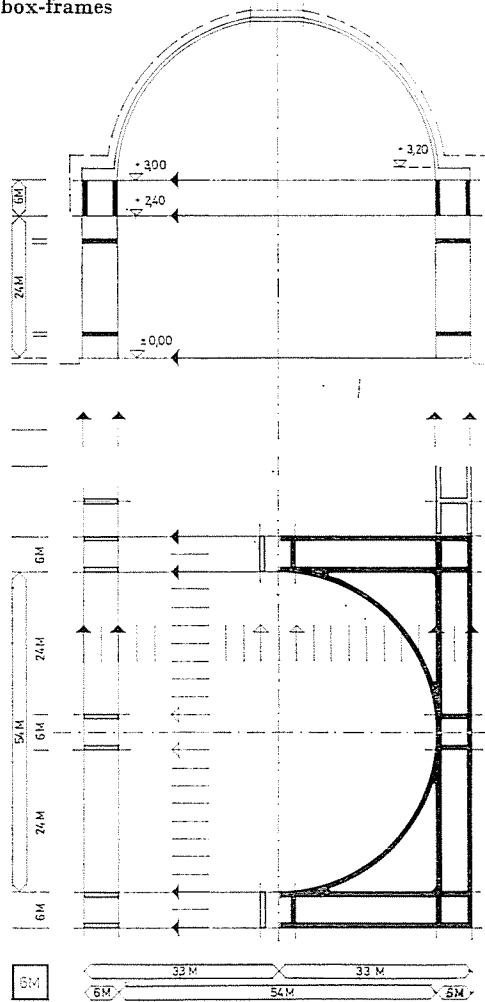
Fig. 28. Location of the domed space in the system of grids on plan and in section. The elements of the dome — the non-tectonic surface elements, the tectonic structural elements, etc. — are always introduced with the respective structural variations
