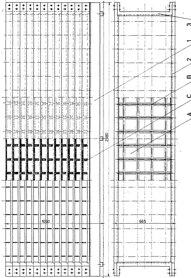
Fig. 18. Stack-plate. Manufacturing apparatus for producing ribbed r.c. shell structural elements. Index: 1. Bottom plate. 2. Longitudinal side profile; 3. Cross profile; A. The non-tectonic periodic gypsum surface element; B. Reinforcement; C. Concrete
