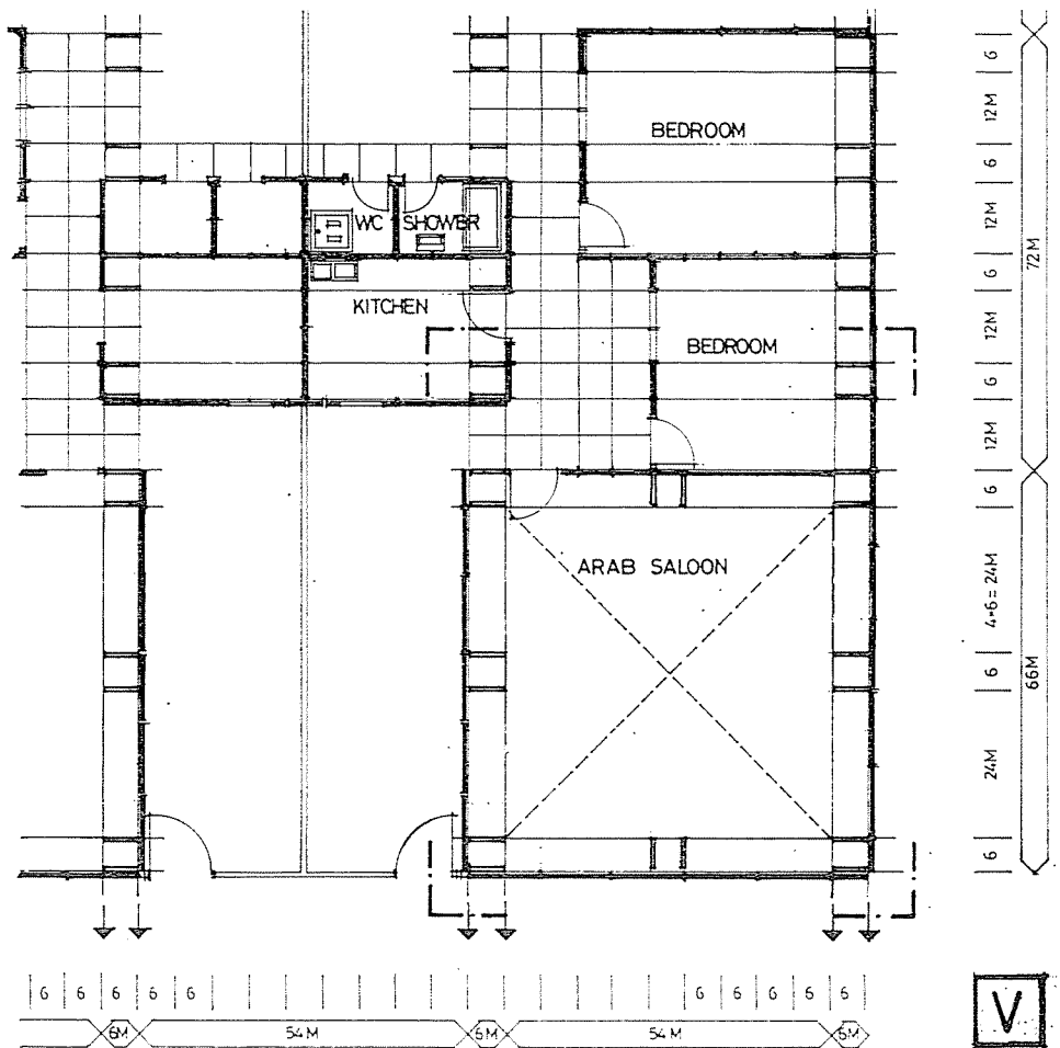
Fig. 9. Location of the vaulted space in the ground plan. From the methodological point of view the adaptation of vaults can most expediently be demonstrated in central-symmetrical arrangements. For this purpose the span dimension (54M) was kept constant, the o/a dimension of pillar-box frames ( 6M \times 6M ) fits into the same zone. Characteristic problems of co-ordination always arise where the one-directional zone of the beam-box-frames meet the central-symmetrical area of the vaults. This is illustrated on the next page by Fig. 10
