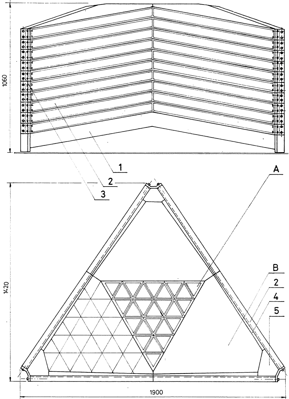
Fig. 35. Ten-unit stack. Manufacturing apparatus for producing ribbed and folded r. c. shell structural small space-units based on the "in-space additivity of non-tectonic elements with plane surface on both sides. Index: 1. Bottom plate; 2. Side profile; 3. Corner element fixing the side; profiles by pairs; 4. Removable inlay pieces for producing elements of different dimensions 5. Inlay element: blocking piece; A. The non-tectonic surface element; B. The concreted small space unit
