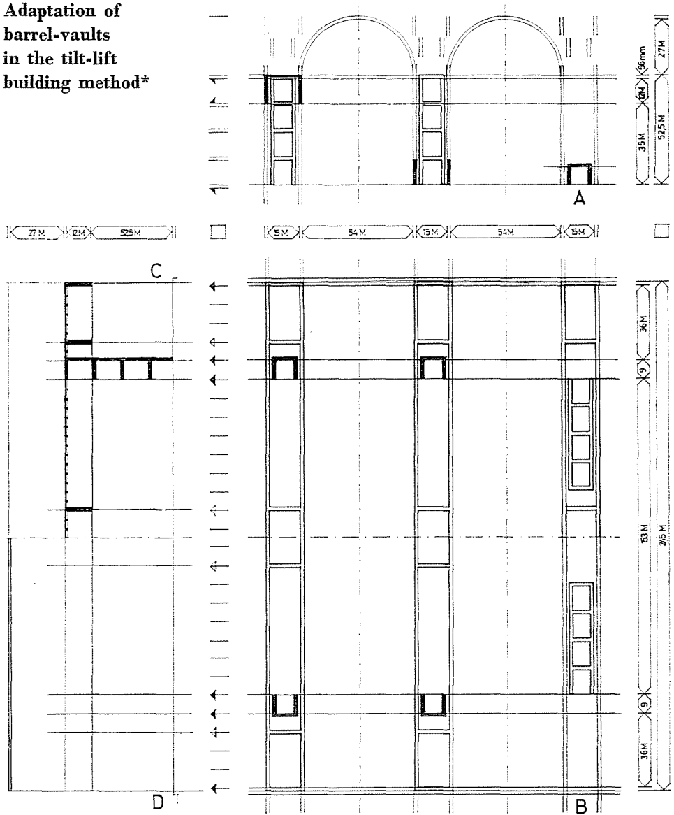
Fig. 42. Location of the barrel-vaulted space in the ground plan and in section. From the methodological point of view the adaptation of barrel-vaults can most expediently be demonstrated if constructed above unbroken longitudinal arrangements and this is why our choice fell on the industrial workshop realized by the tilt-lift building method. Figure 42. and Fig. 43 show a repetitive structural unit on plan and in section. Index: A. Cross-sections, situations prior to and after tilting and lifting; B. Plan. Situations prior to and after tilting and lifting; C. Longitudinal section through beam box-frame; D. Longitudinal section through barrel-vault
