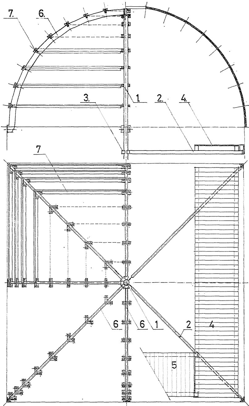
Fig. 14. Auxiliary structure for the assembly of cloister vault. Index: 1. Leading post started from the zero-level of co-ordination; 2. Stiffening and supporting rod; 3. Welded collar; 4. "Gang-way". Timber running-board supported by the diagonal stiffening rods; 5. The same, supported by the running-board 4.; Poligonal supporting arch; 7. Shuttering rods jointed to supporting arch 5
