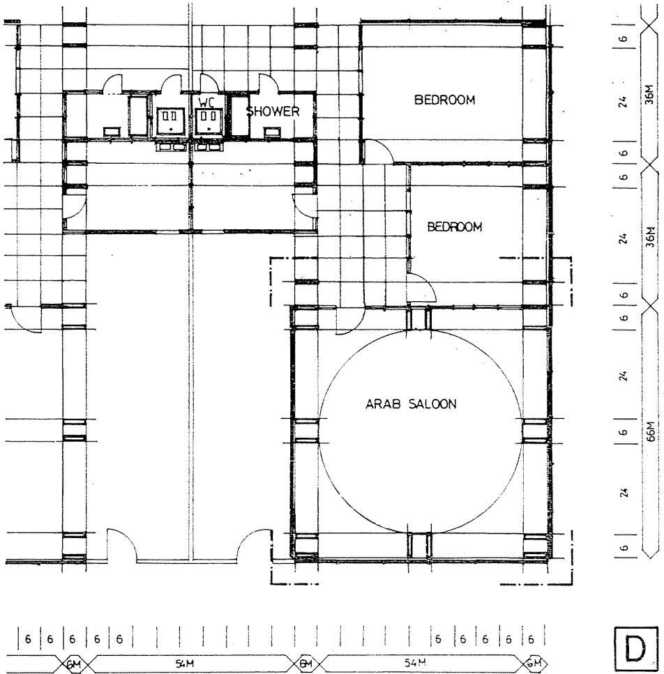
Fig. 27. Location of the domed space in the ground plan. From the methodological point of view the adaptation of domes can most expediently be demonstrated in central-symmetrical arrangements. For this purpose the span dimension (54M) is kept constant, the o/a dimensions of pillar-box-frames (6M × 6M; 6M × 12M; 6M × 12M + mc) are variable but they always fit into the 6M zone. Characteristic problems of co-ordination always arise where the one-directional zone of the closed cellular floor-fields meet the central-symmetrical area of the dome, as illustrated by Fig. 28
