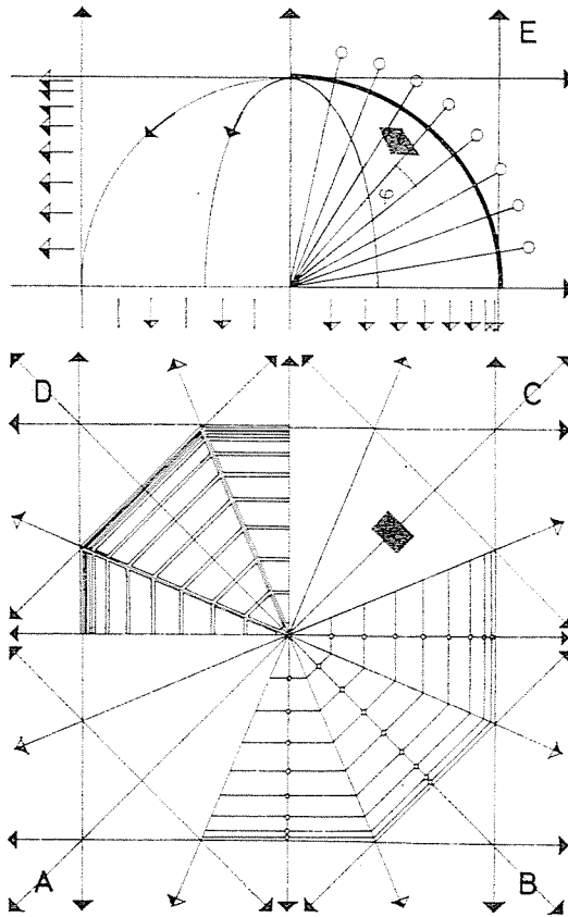
Fig. 21. The system of grids of variation V. 4. on plan and in section. Decomposition of the structure
