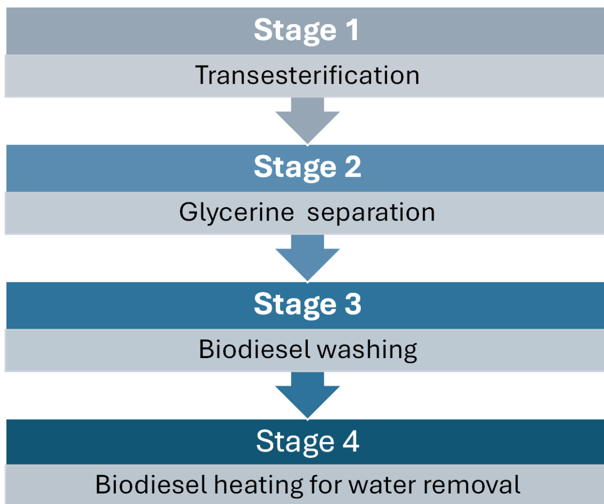
Fig. S1 Schematic diagram of stage-wise production of biodiesel from jojoba oil
