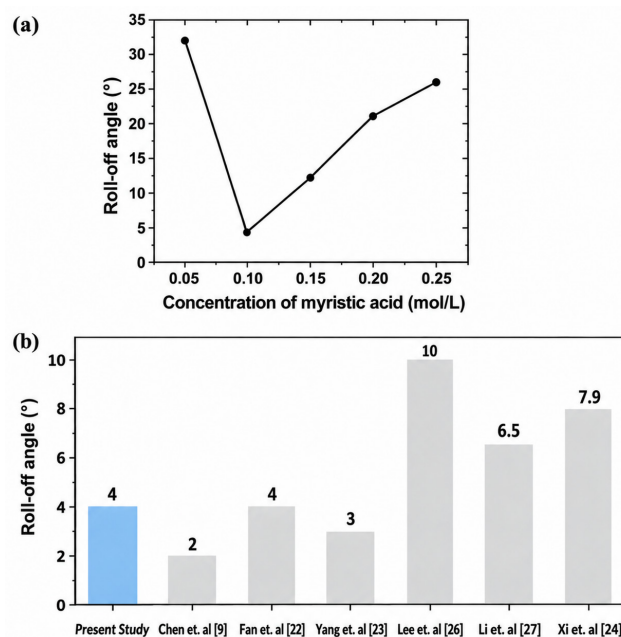
Fig. 8 (a) Variation of roll-off angle with MTA concentration showing minimum roll-off at 0.1 M. (b) Comparative roll-off angles of the present coating with previously reported superhydrophobic surfaces from literature [9, 22–24, 26, 27].
