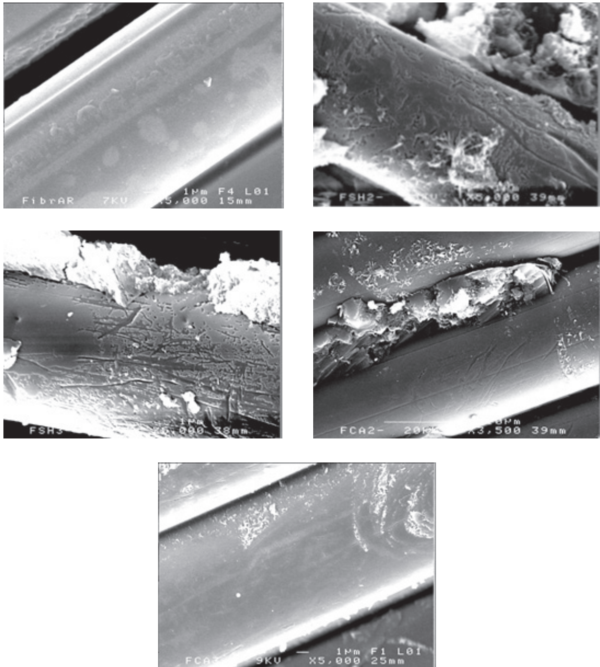
Fig. 4 SEM observations of the CemFil fiber (A.R.) before mixing and of the glass fibers in the CEM II/B 32:5 cement matrix, conserved in different environments
