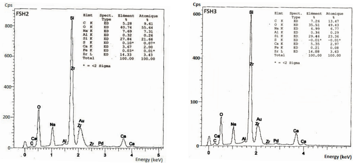
Fig. 5 Spectrometry X-ray analyses of the fibre body of GFRC cured in moist room
