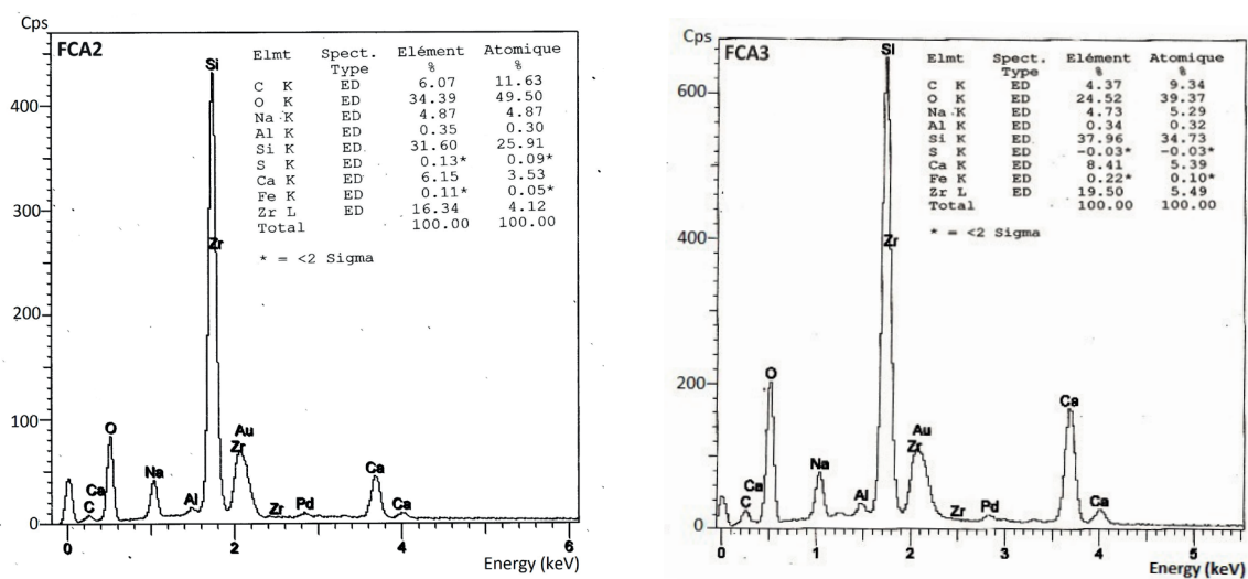
Fig. 6 Spectrometry X-ray analyses of the fibre body of GFRC cured at ambient air
