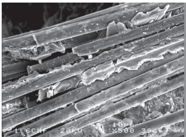
Fig. 2 Filling of the spaces between the filaments by calcium hydroxide. Note surface corrosion and notching by Ca(OH) 2
