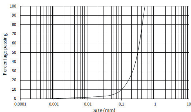
Fig. 1 Particle size distribution of sand
