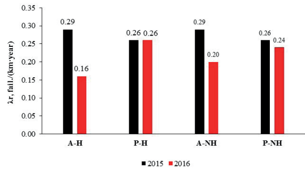
Fig. 2 Real and predicted values of failure rate of distribution pipes
