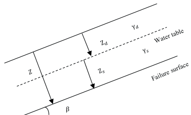
Fig. 6 The slope with translational slip
