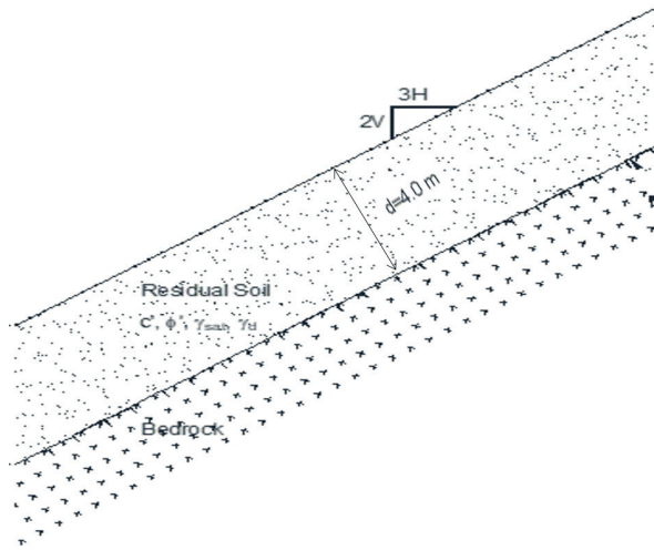
Fig. 8 A residual soil slope
