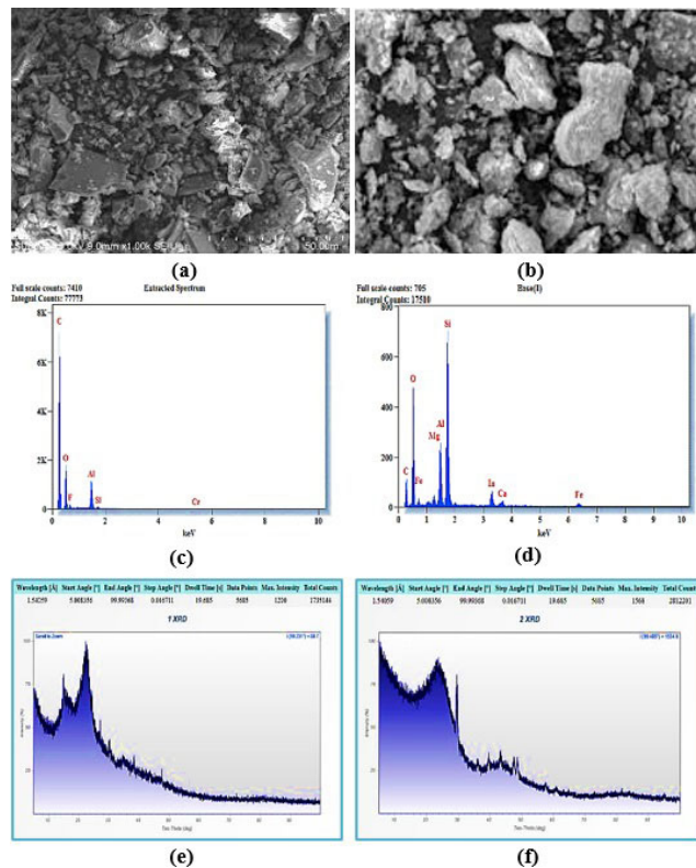
Fig. 13 Microstructure analysis of self-healing concrete by (a) Normal mix and (b) Bacterial Concrete, by EDX for (c) Normal mix and (d) Bacterial Concrete and by XRD for (e) Normal mix and (f) Bacterial concrete respectively
