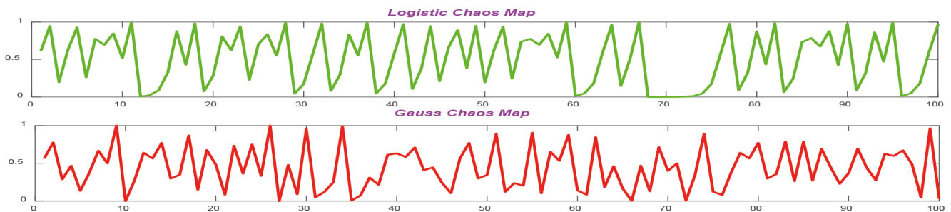
Fig. 2 The chaotic value distribution during 100 iterations
