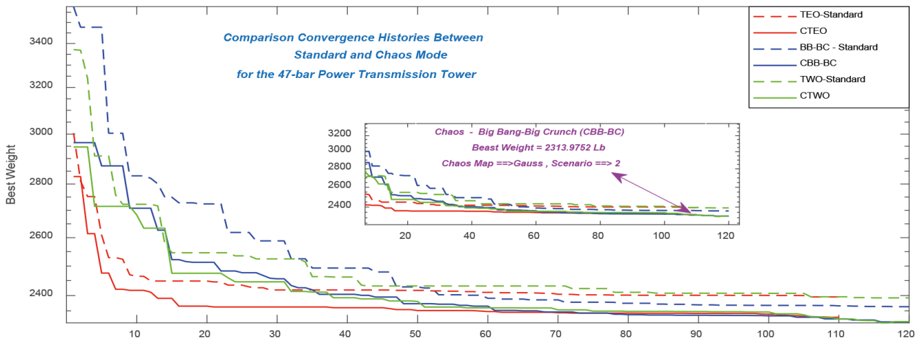
Fig. 5 The convergence histories for the 47-bar power transmission tower
