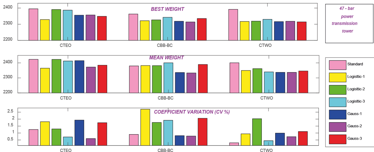
Fig. 4 Optimization results in standard mode and selection of chaos map for the 47-bar power transmission tower
