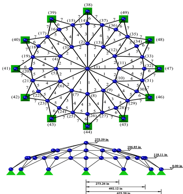
Fig. 6 Schematic of a 120-bar dome shaped truss
