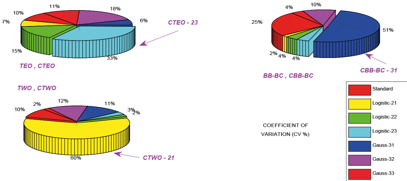
Fig. 11 The final results of the optimal design to determine the best coefficient of variation
