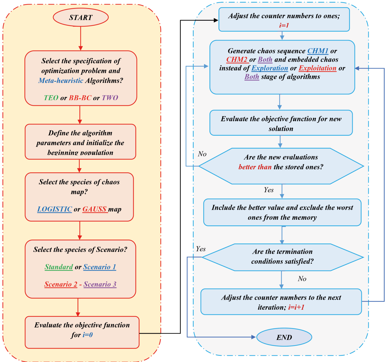
Fig. 1 Flowchart for the chaos algorithm
