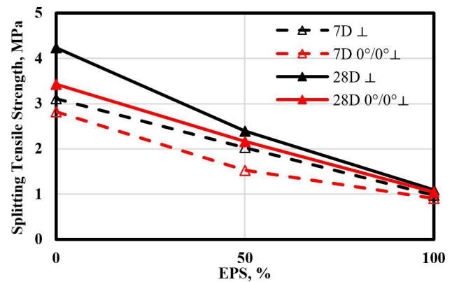
Fig. 12 Splitting tensile strength of casted ( \perp ) and printed ( 0^\circ/0^\circ \perp ) specimens
