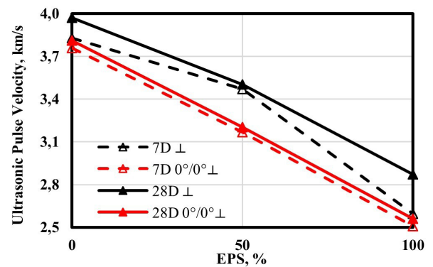
Fig. 9 Ultrasonic pulse velocities of casted ( \perp ) and printed (0°/0° \perp ) specimens
