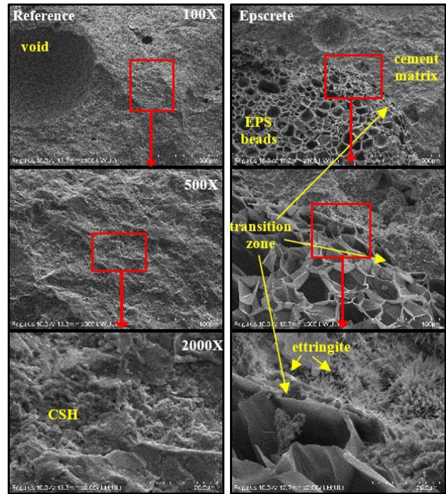
Fig. 18 Micrograph of epscrete and reference samples
