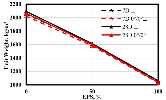
Fig. 8 Unit weights of casted ( \perp ) and printed (0°/0° \perp ) specimens containing EPS
