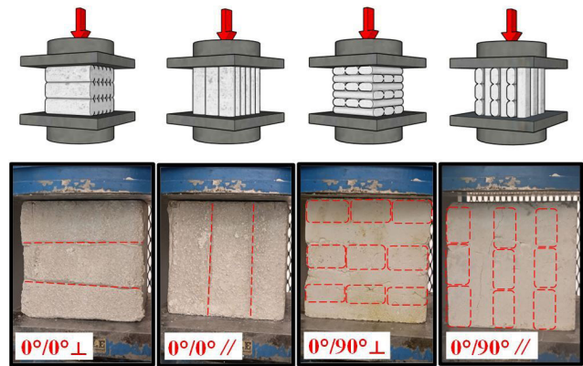
Fig. 5 Compressive strength tests according to different loading and printing directions
