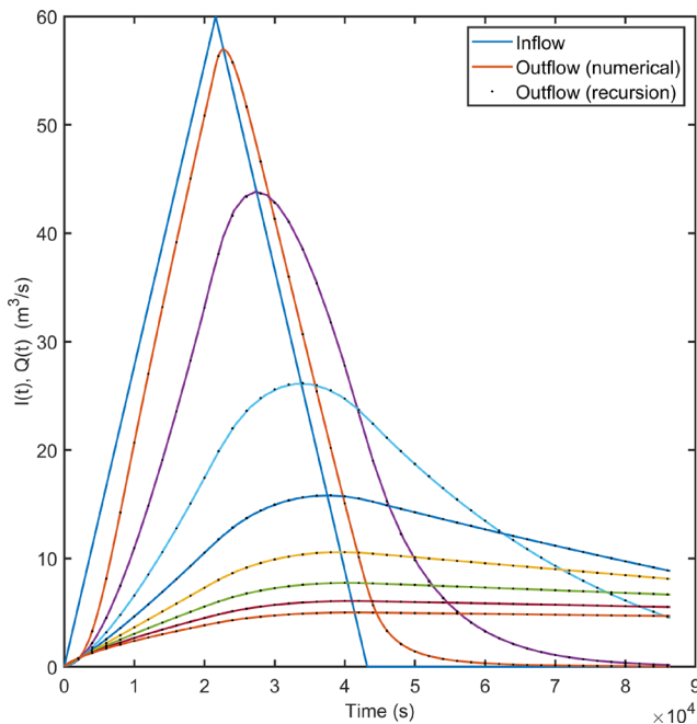
Fig. 1 Comparison of the recursive solution [Eq. (10) plotted at 200 dt s time increments] of Eq. (4), to one obtained by numerical integration for different values of m incremented by 0.5
