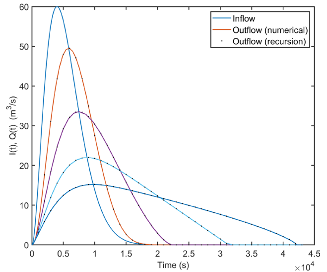
Fig. 2 Comparison of the recursive solution [Eq. (10) plotted at 100 dt s time increments] of Eq. (4) to one obtained by numerical integration for different values of m incremented by 0.5
