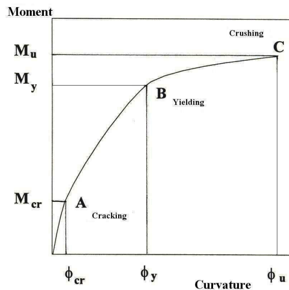
Fig. 1. Qualitative moment-curvature relationship
