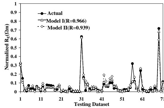
Fig. 4. Performance of testing dataset.
