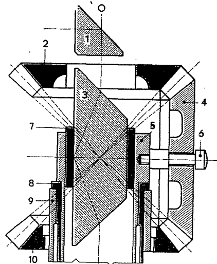
Fig 17. The Dowe erecting prism controlled by differential gear
