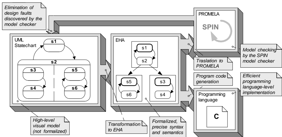
Fig. 13. Model checking and automatic code generation unified in a single framework
