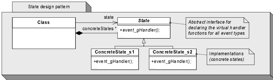
Fig. 6. Implementation by the State design pattern
