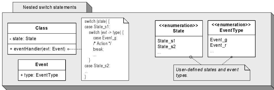
Fig. 4. Implementation by nested switch statements
