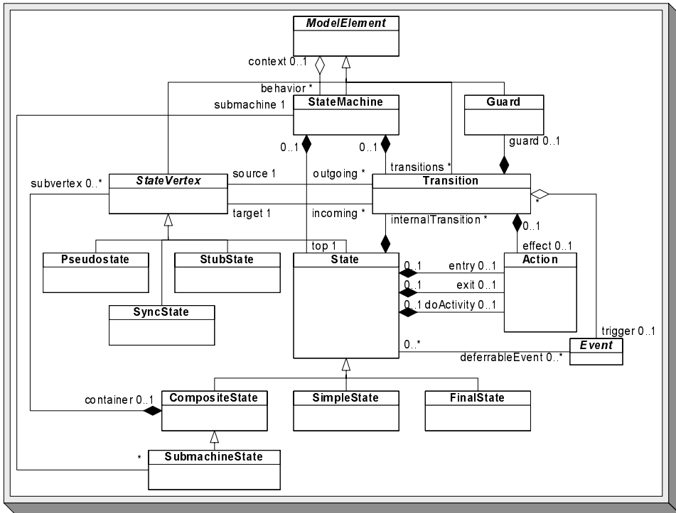
Fig. 2. Metamodel of UML statecharts [10]
