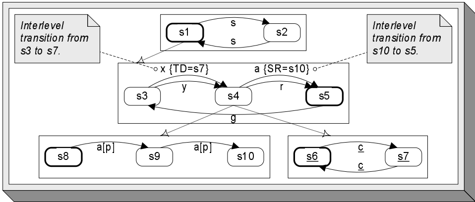
Fig. 11. EHA representation of the example UML statechart
