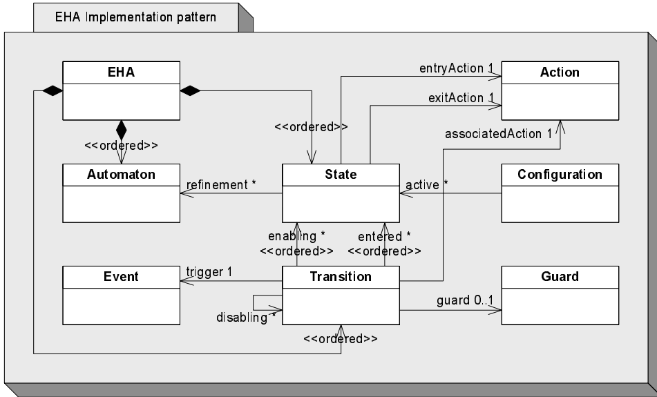
Fig. 12. Class diagram of the proposed pattern
