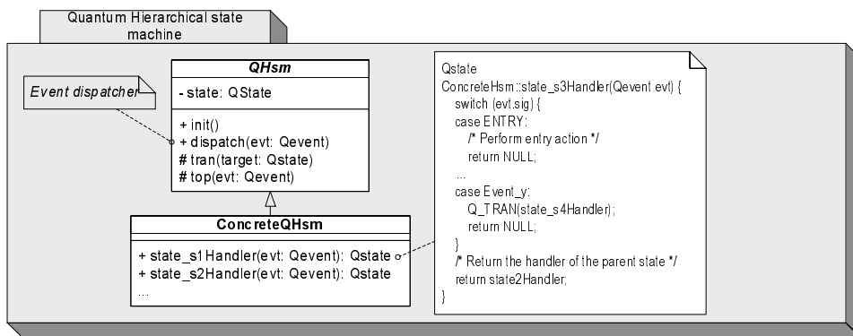
Fig. 7. Implementation by Quantum Hierarchical state machine
