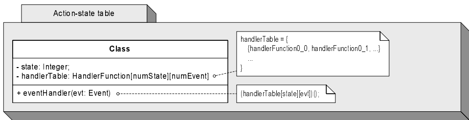
Fig. 5. Implementation by action-state tables
