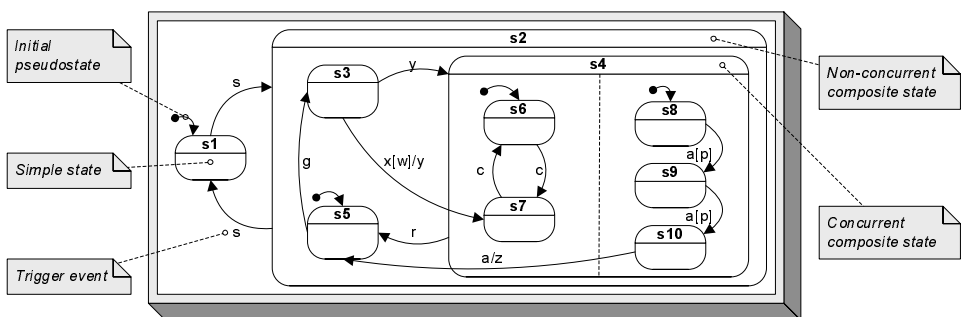
Fig. 3. Example of a UML statechart diagram
