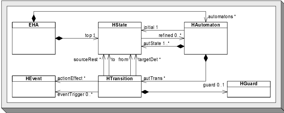
Fig. 10. Metamodel of Extended Hierarchical Automata
