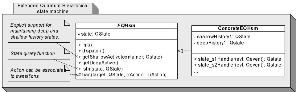
Fig. 8. Implementation by the Extended Quantum Hierarchical state machine
