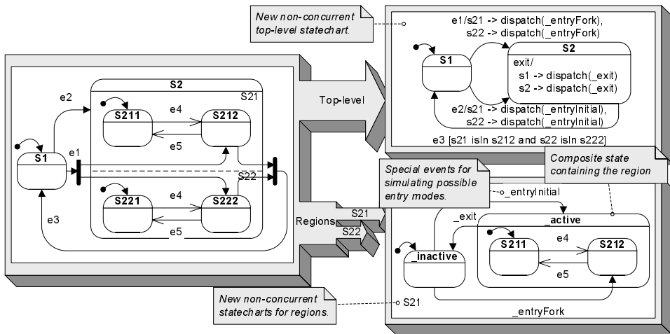
Fig. 9. Decomposition of concurrent composite states into individual state machines
