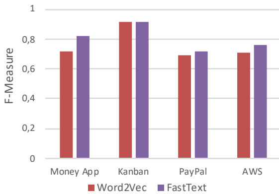
Fig. 2 Performance of Word2Vec vs fastText
