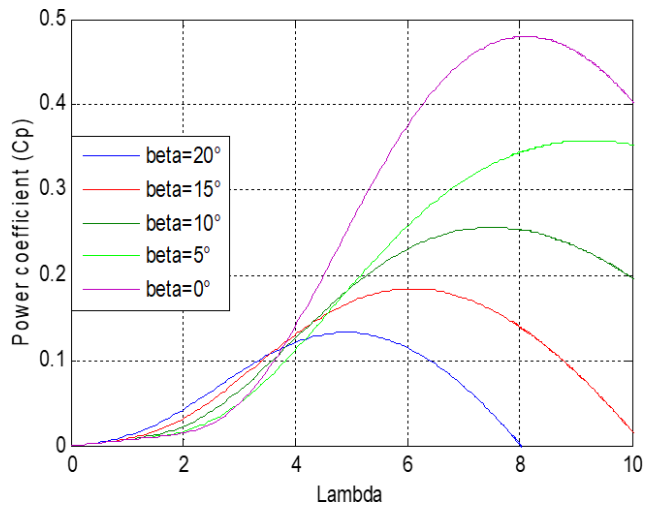
Fig. 4 Characteristic curves C_p(\lambda) ( \beta , expressed in degree)
