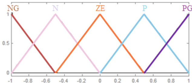
Fig. 6 Memberships functions of ( e , de ) and duty cycle for WECs and pitch angle controllers
