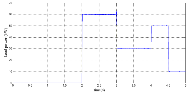
Fig. 11 Load power
