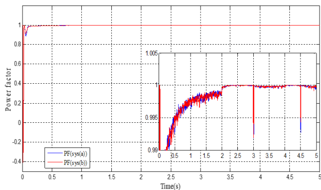
Fig. 20 Power factor
