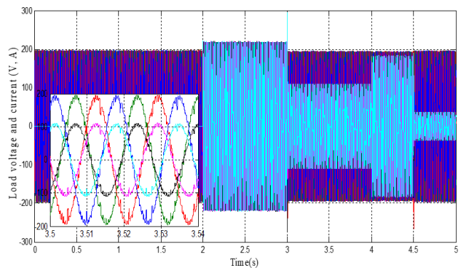
Fig. 18 Load voltage and current
