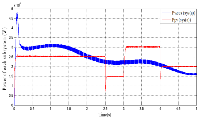
Fig. 14 Powers of subsystem (a)
