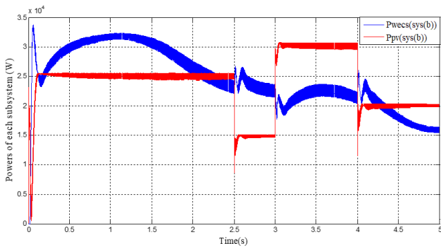
Fig. 15 Powers of the subsystem (b)
