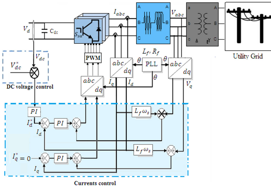
Fig. 8 Inverter control
