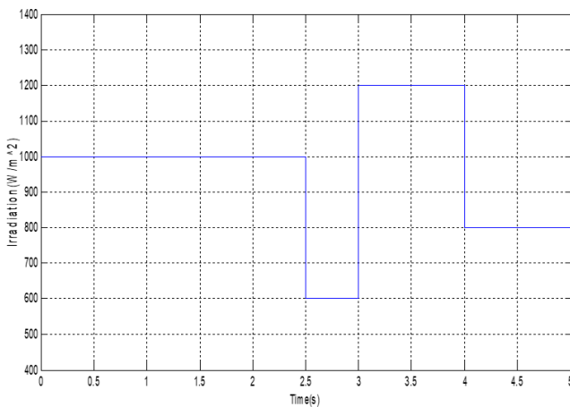
Fig. 9 Irradiation profile
