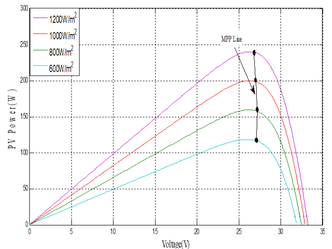
Fig. 3 PV characteristics
