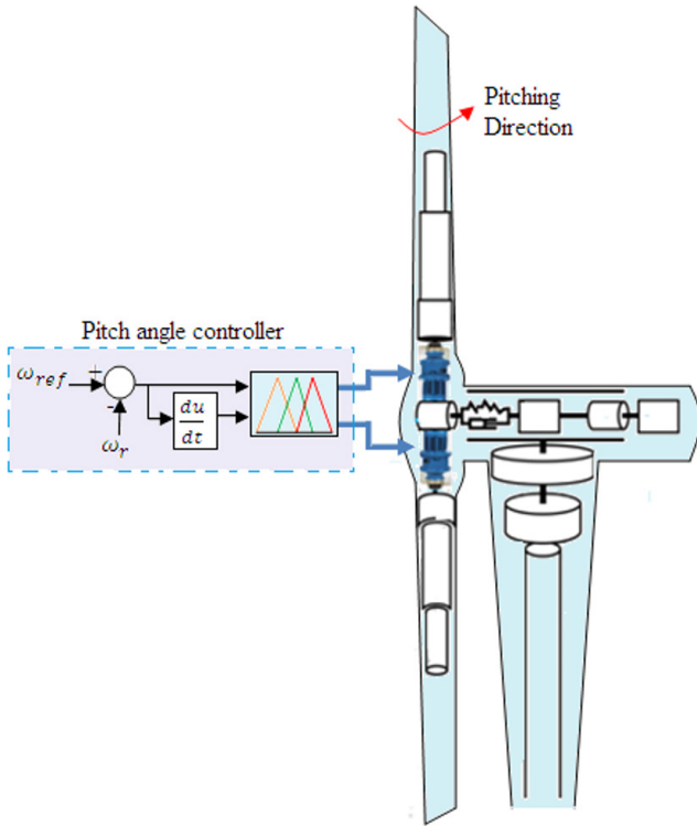
Fig. 5 Pitch angle control
