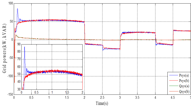
Fig. 13 Grid powers of each system
