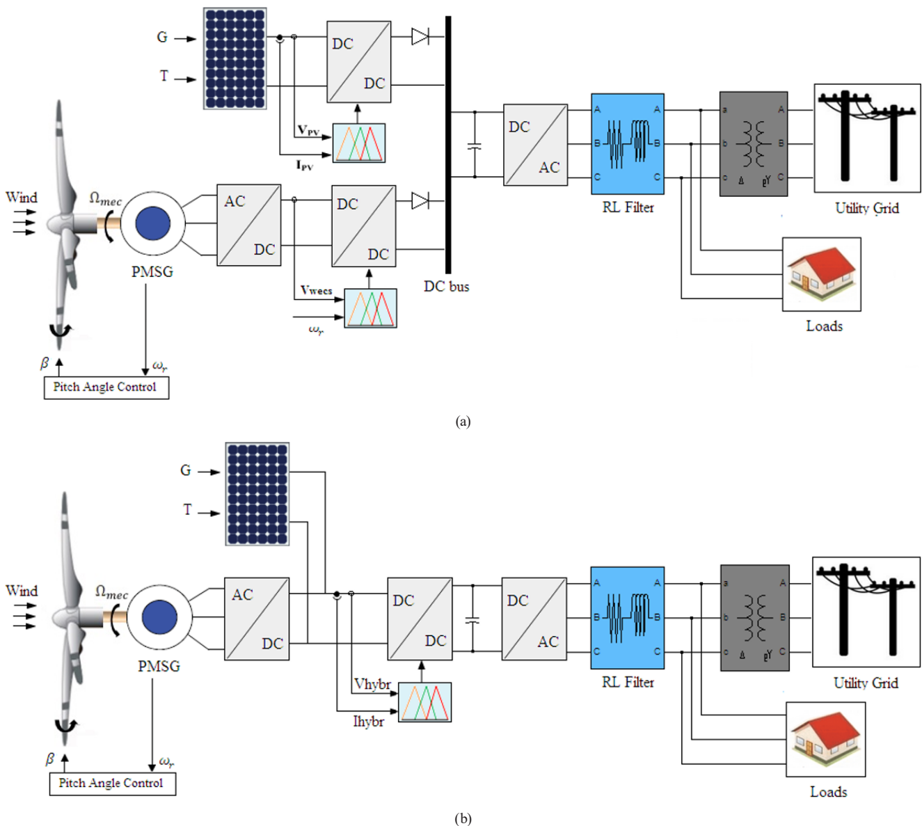
Fig. 1 Hybridization Topologies: (a) individuals MPPT, (b) common MPPT
