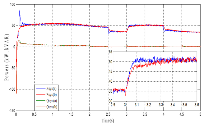
Fig. 12 Inverter powers of each system
