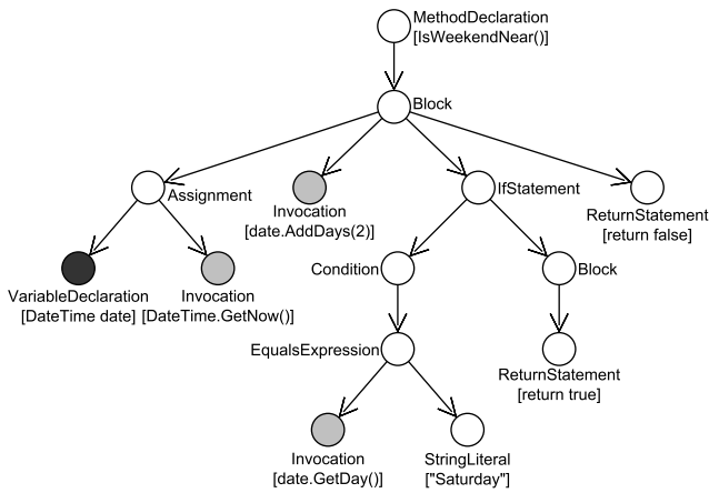
Fig. 1 The simplified AST of method IsWeekendNear
