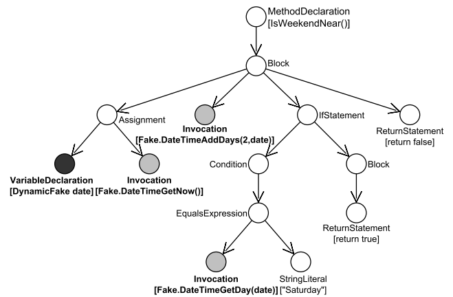
Fig. 2 The transformed AST of method IsWeekendNear
