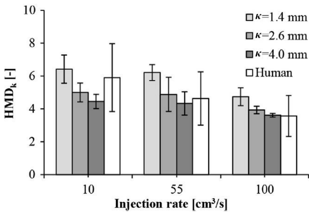
Fig. 5 Inhomogeneity as a function of injection rate
