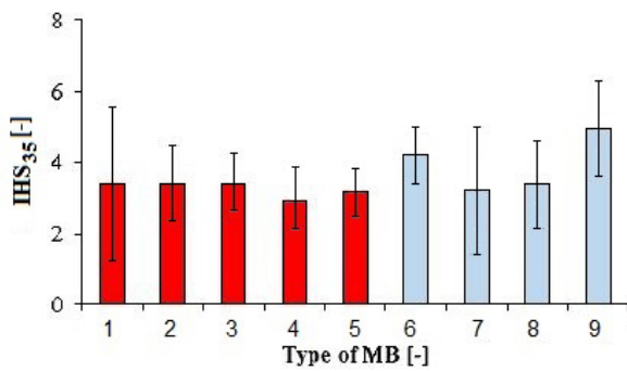
Fig. 14 Inhomogeneity of various monobatches
