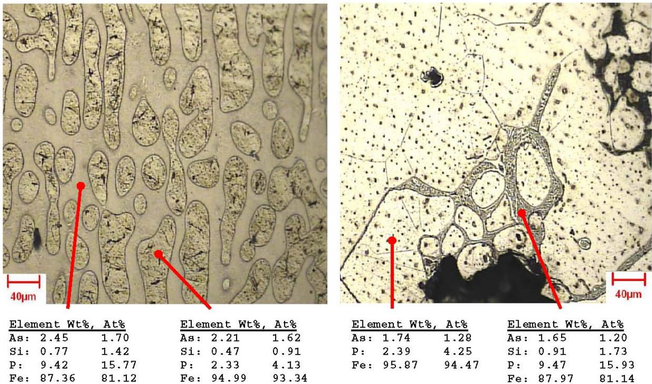
Fig. 4. Metallographic picture of iron bloom samples (200x). a) iron bloom made of Fancsika iron ore b) iron bloom made of Petesmalom iron ore.
