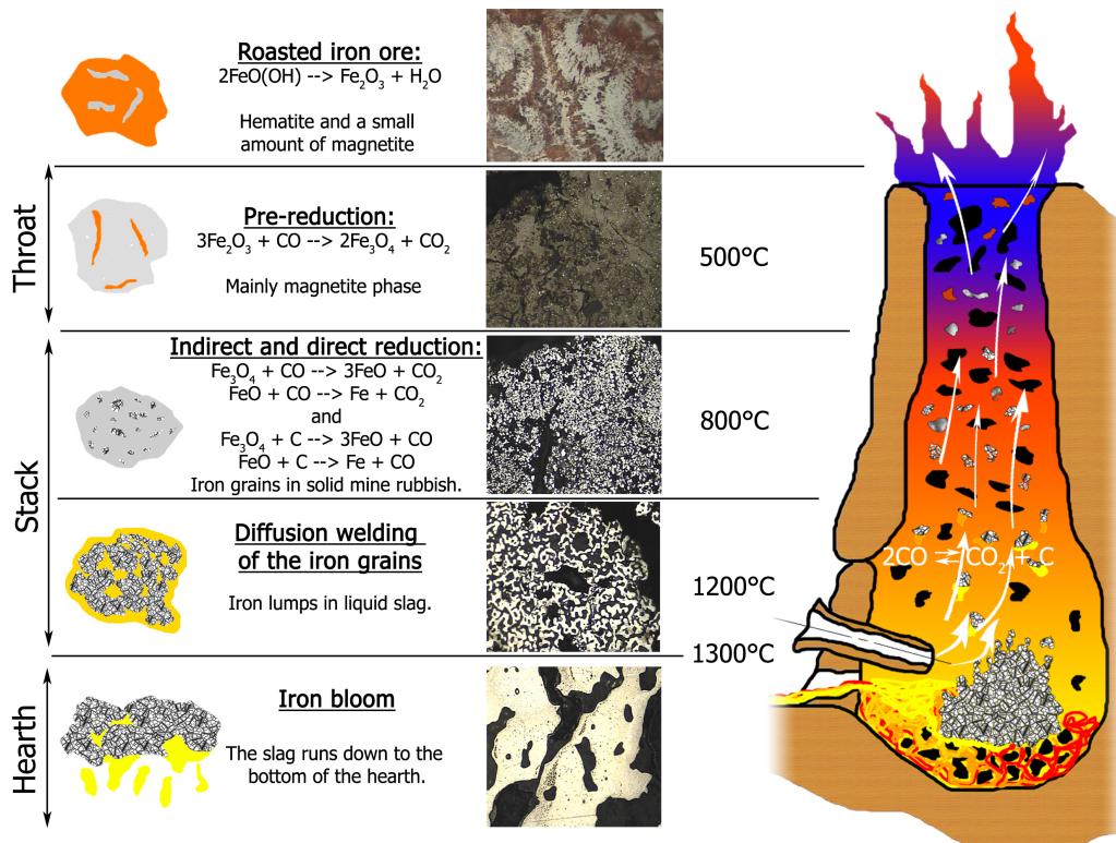
Fig. 5. The metallurgy of the bloomery.
