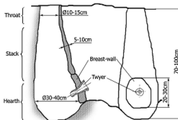
Fig. 1. Typical construction and dimensions of the Fajszi-type bloomery.
