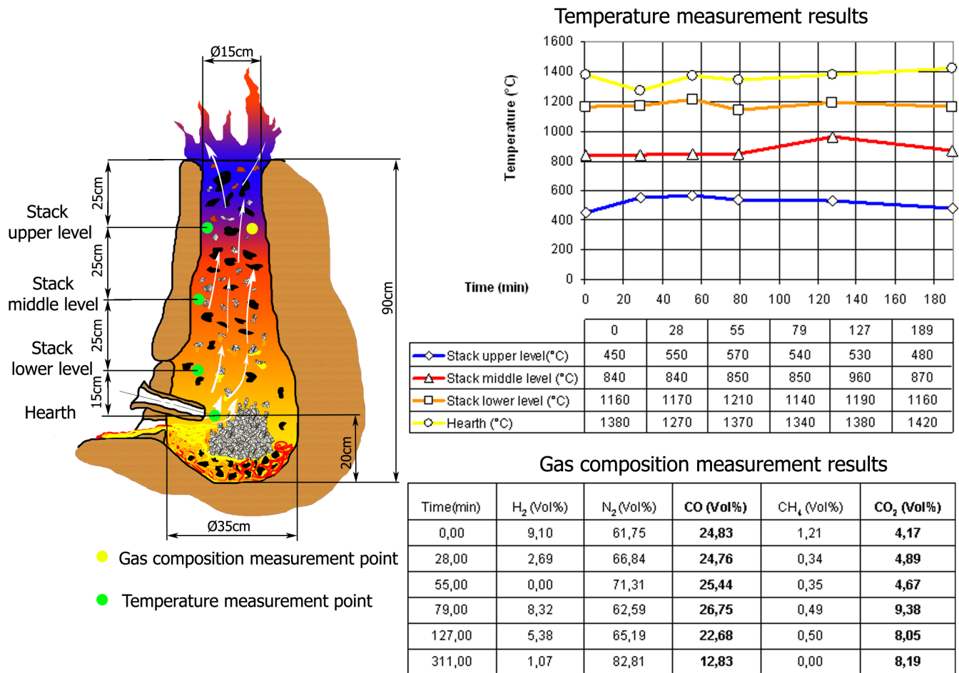
Fig. 3. Temperature and gas composition measurement points in the furnace and the results.
