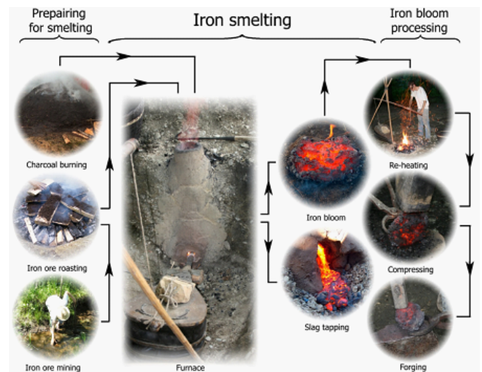
Fig. 2. The steps of the early medieval iron manufacturing.
