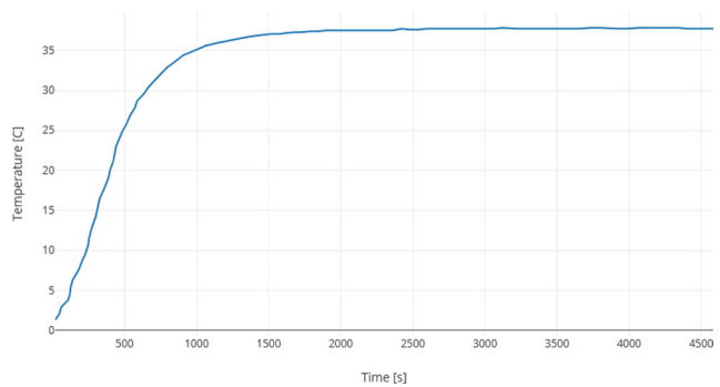
Fig. 8 The relationship between water temperature and time with fuzzy control mode of the geothermal-source heat pump system
