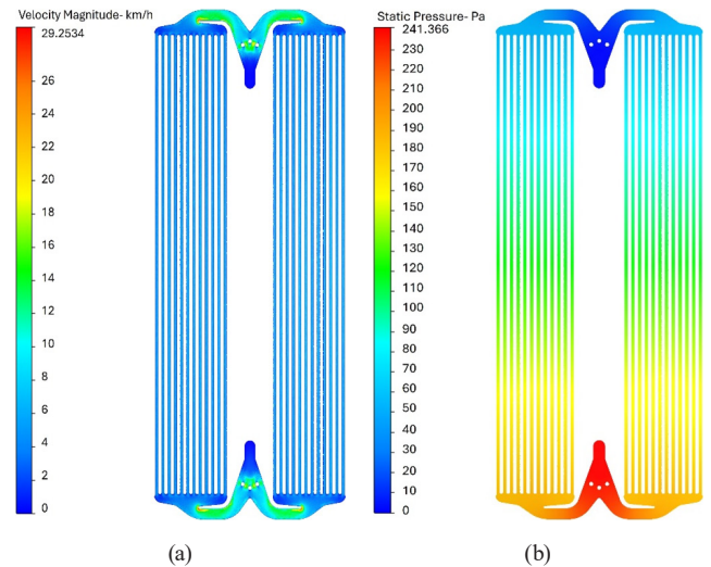
Fig. 6 V3 anode side (a) velocity distribution and (b) pressure distribution
