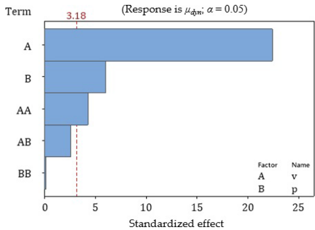
Fig. 4 Results of the significance test of the factors affecting the dynamic friction coefficient ( \mu_{dyn} )
