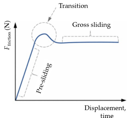
Fig. 1 Schematic friction-force curve as a function of time or displacement
