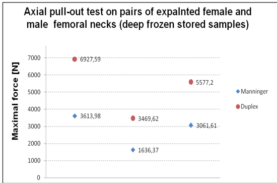
Fig. 14 On the left: 1st pair: a male's bone, Manning's screw 8 vs. duplex screw; 2nd pair: a particularly old male, Manning's screw 9.5 vs. duplex screw; 3rd pair: female bone, Manning's screw 8 vs. duplex screw. On the right: 1st pair: a male's bone, Manning's screw 8 vs. duplex screw; 2nd pair: a particularly old male, Manning's screw 9.5 vs. duplex screw; 3rd pair: female bone, Manning's screw 8 vs. duplex screw
