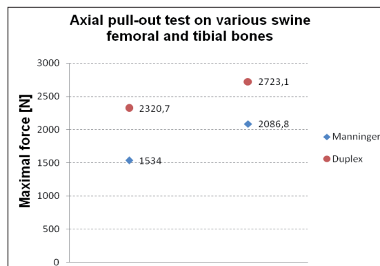
Fig. 13 Experiments on mixed bones
