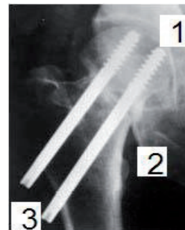
Fig. 1 Fixation of fracture of the neck of the femur by duplex canulated screwing
