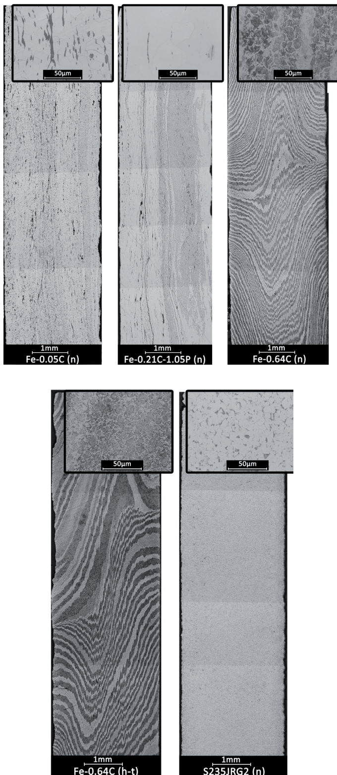
Fig. 1 Metallographic macro-photographs of cross-sections of representative specimens of each type
