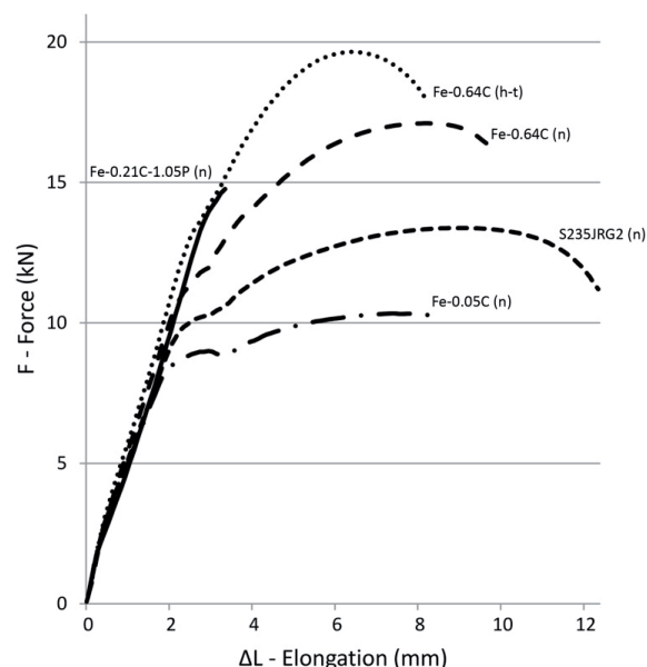
Fig. 2 Tensile diagram of representative samples of each type
