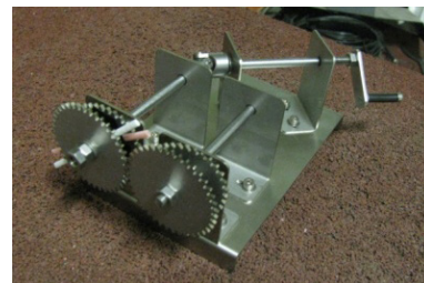
Fig. 3 Device that eliminates the angular velocity alternation of a 45° deflected cardan joint [8].
