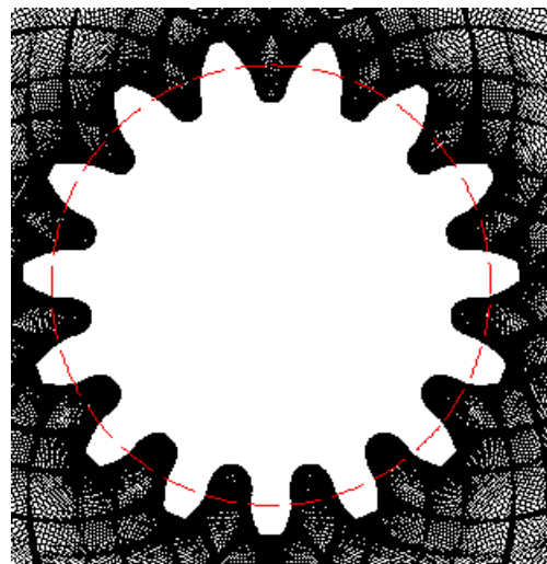
Fig. 6 Changing ratio cylindrical gears with a 3° amplitude sine function like angle alternation and different numbers of teeth.
