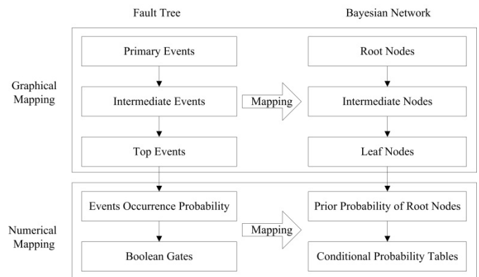
Fig. 3 Transformation flow chart from FT to BN.
