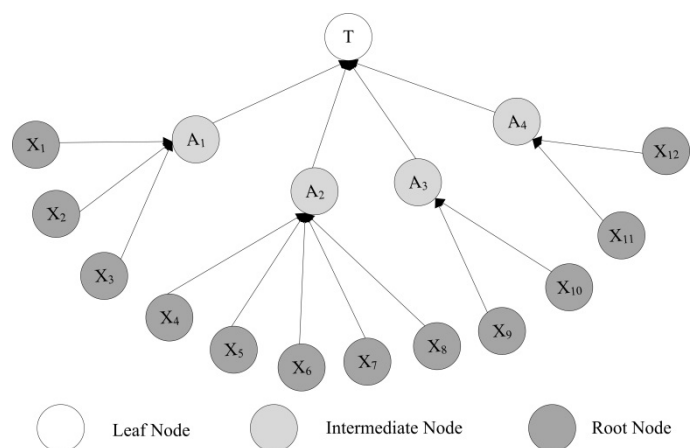
Fig. 4 Established Bayesian network model for RPTS
