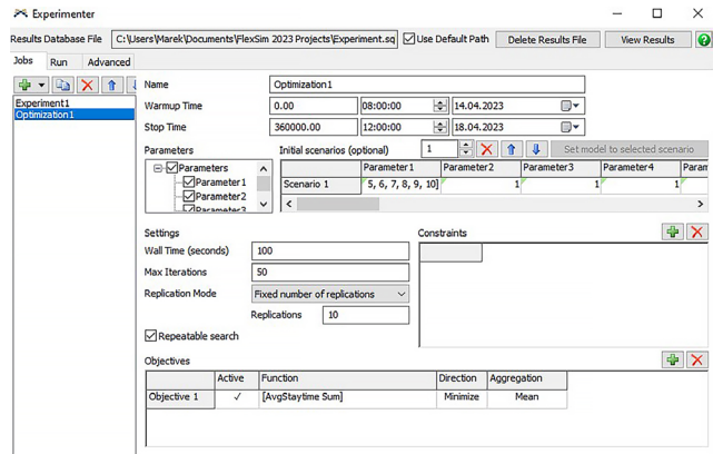
Fig. 7 The settings of the FlexSim Optimizer
