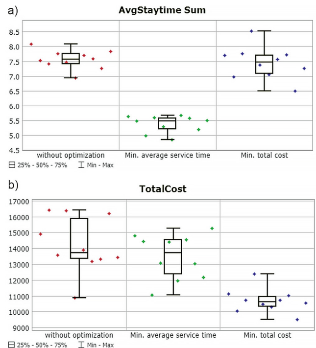
Fig. 8 Confidence intervals for: a) average service time [h], b) service costs [monetary units]
