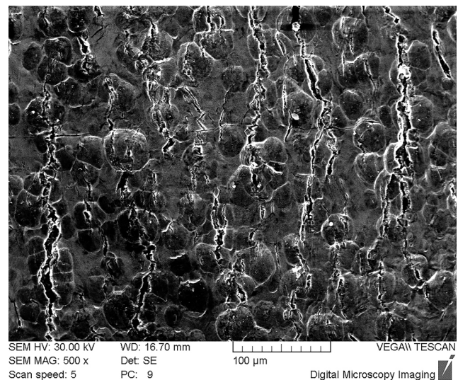
Fig. 4 SEM image of cracked coating (a) and EDX microanalysis in the same area (b)
