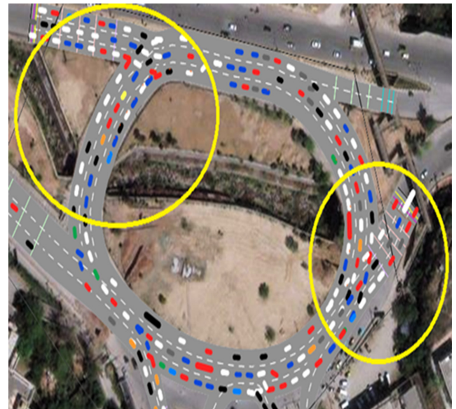
Fig. 6 Traffic congestion situation using PTV Vissim software
